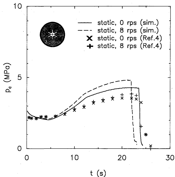
Fig. 1 Predicted pressure-time histories for static firing of motor A, with comparison to firing data of Ref. 4.
